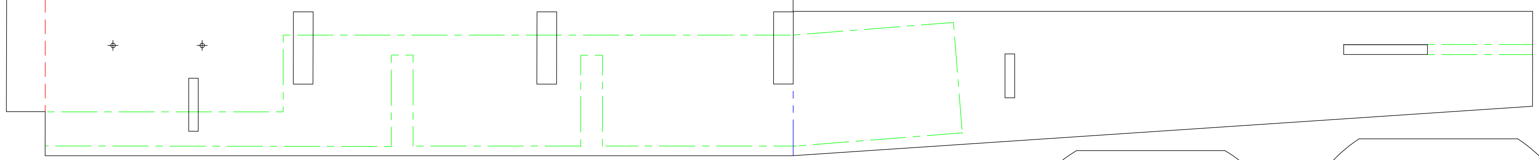
15 MIDDLE - BACK? 1 FOAM BOARD LOCKHEED VEGA - V.1.0
