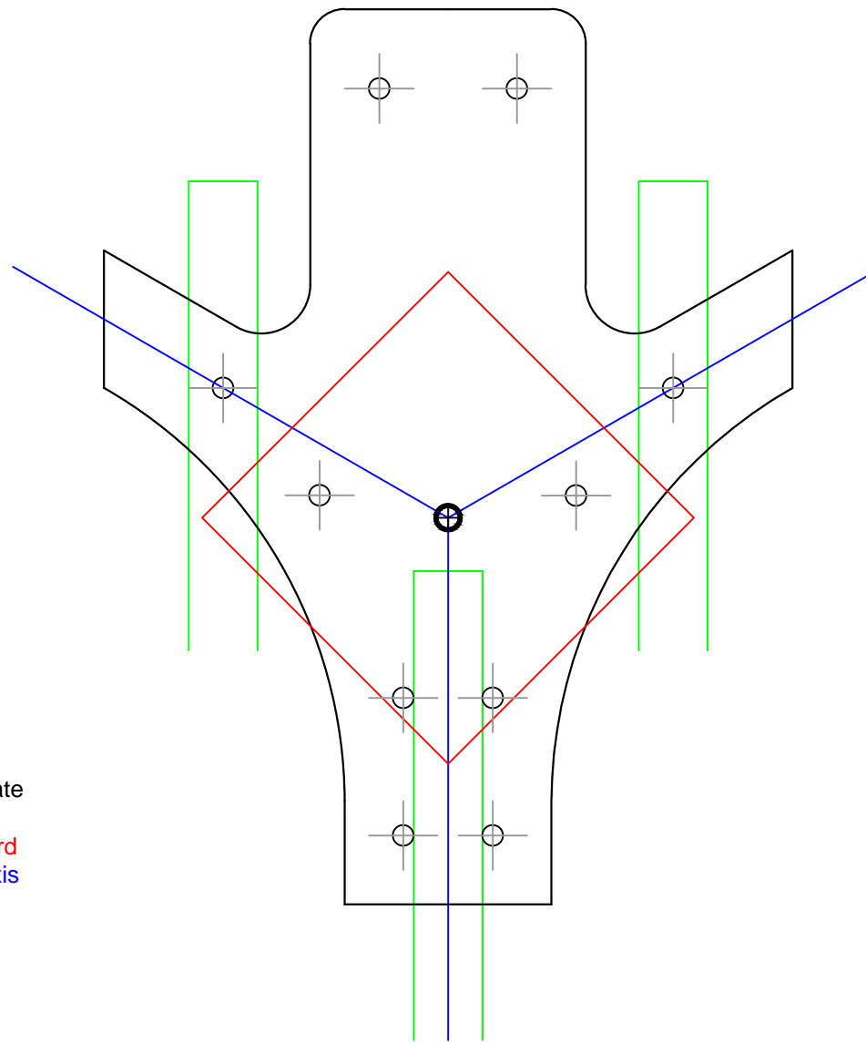
Unfolded Arms
