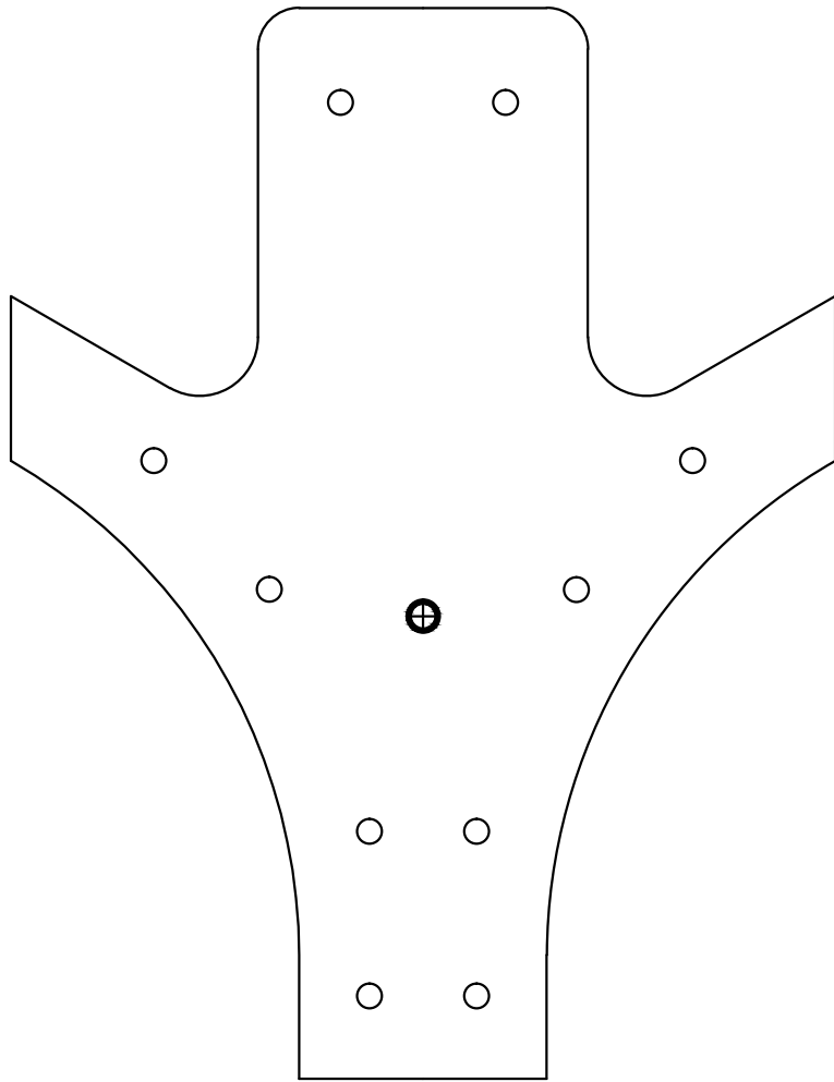
RCExplorer.se Tricopter Suggested Template
